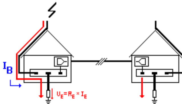
FIG 1. Directly Coupled
