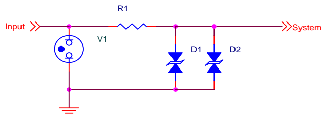
FIG. 12 Multi-Component Suppressor
