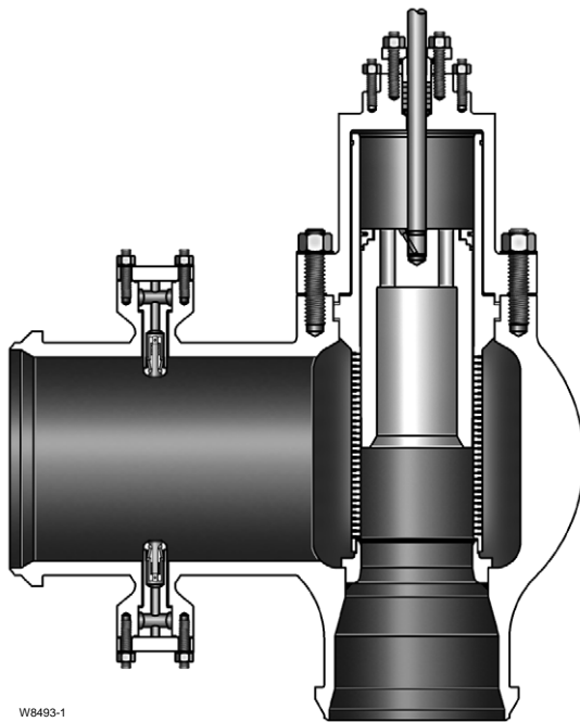
Figure 7-9. Cross-Section View of Steam Conditioning Valve
