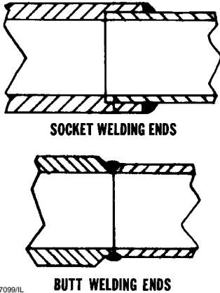
Figure 3-14. Common Welded End Connections
