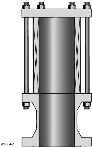
Figure 7-13. Steam Sparger Utilizing Multi-Stage Pressure Drop Technique
